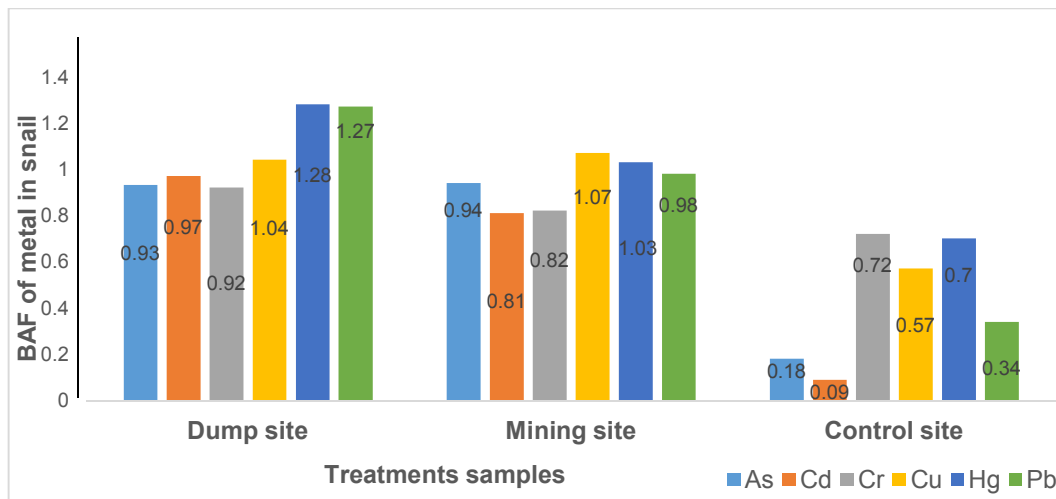
Fig. 1. Bioaccumulation factor of metals in snail
