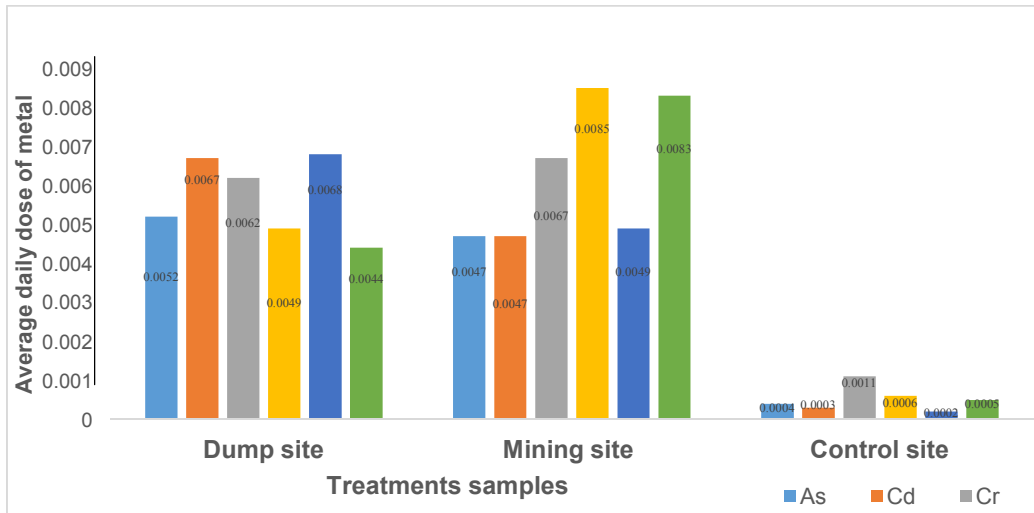
Fig. 2. Estimation of average daily dose of metal for adult
