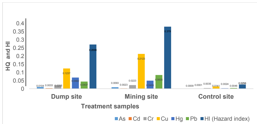
Fig. 3. Estimation of hazard quotient and hazard index
