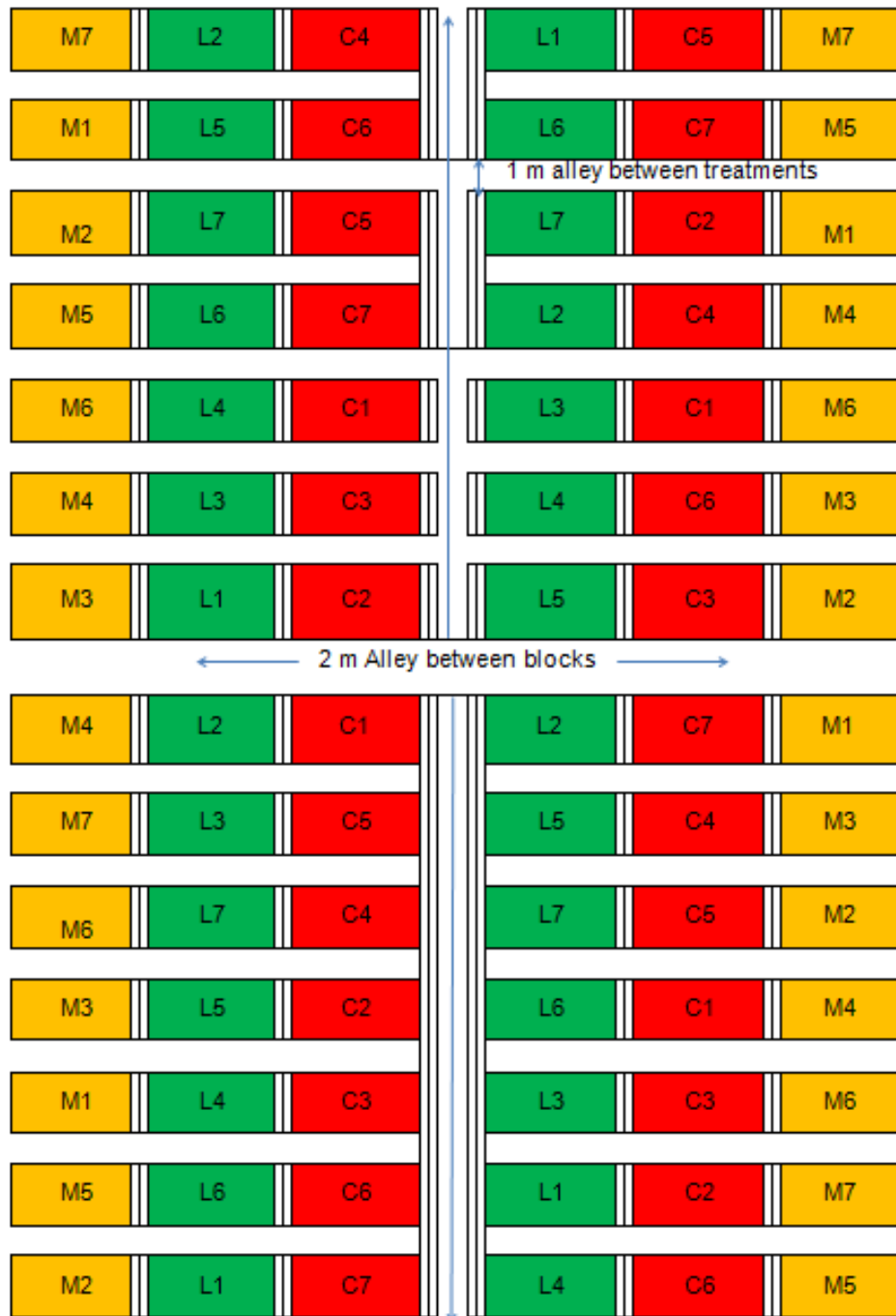
Fig. 3. Layout of maize field experiment at Wang'waray FTC
