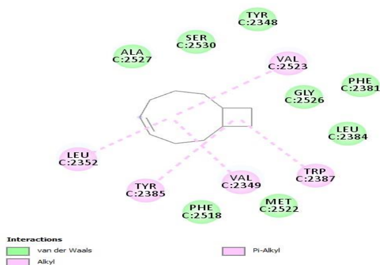
Fig. 1. Interaction of the protein with Bicyclo[7.2.0]undec-4-ene.
