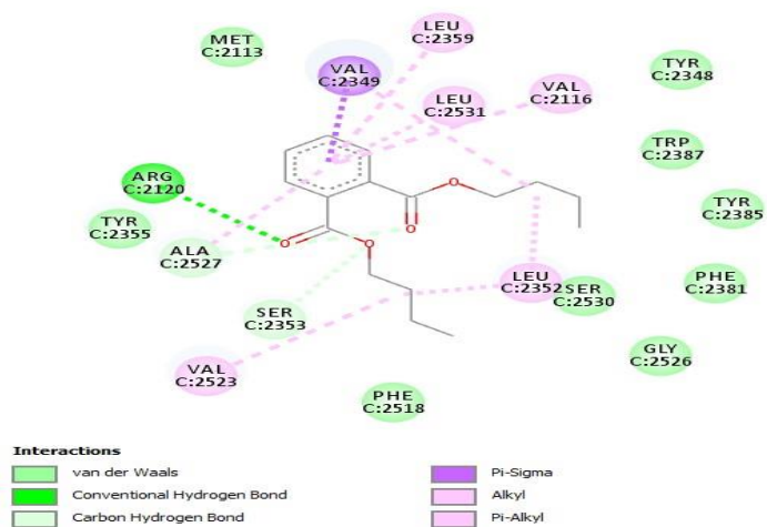
Fig. 3. Interaction of the protein with Dibutyl phthalate
