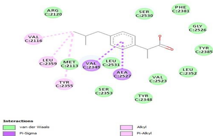
Fig. 5. Interaction of the protein with Ibuprofen
