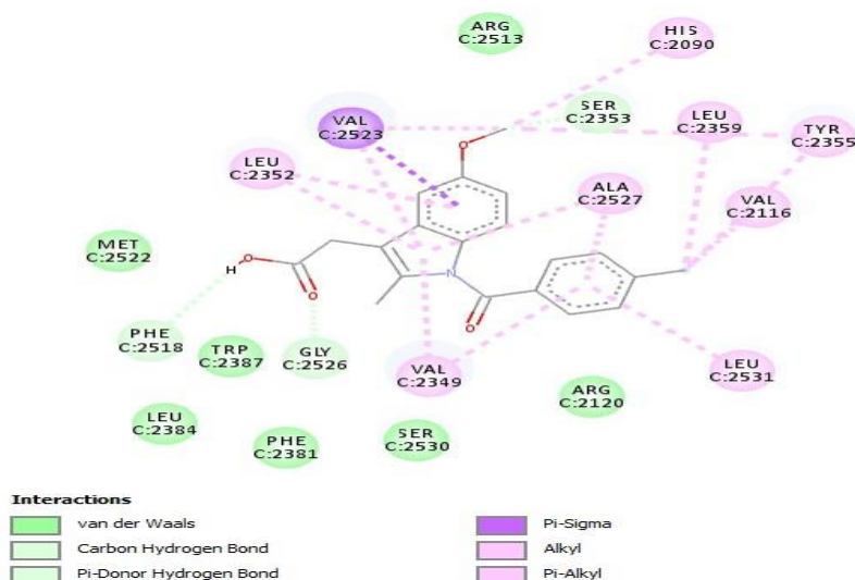
Fig. 6. Interaction of the protein with indomethacin
