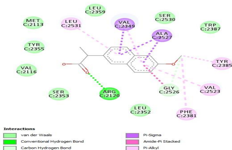
Fig. 7. Interaction of the protein with Naproxen
