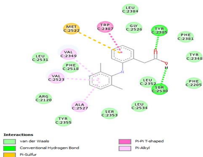
Fig. 4. Interaction of the protein with Diclofenac
