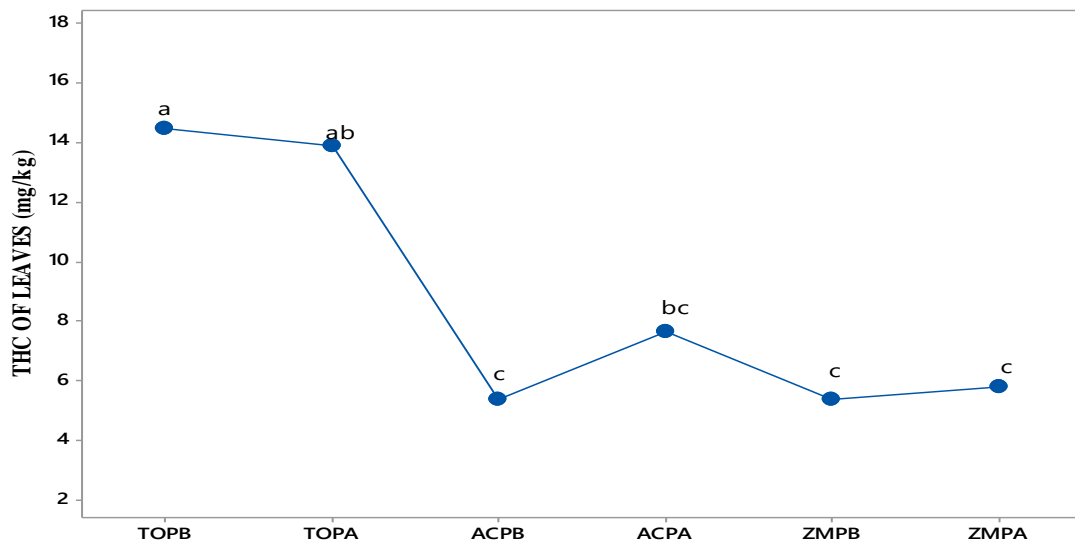
Fig. 5. Total hydrocarbon content for polluted test plants at day 14 according to their pollution time
