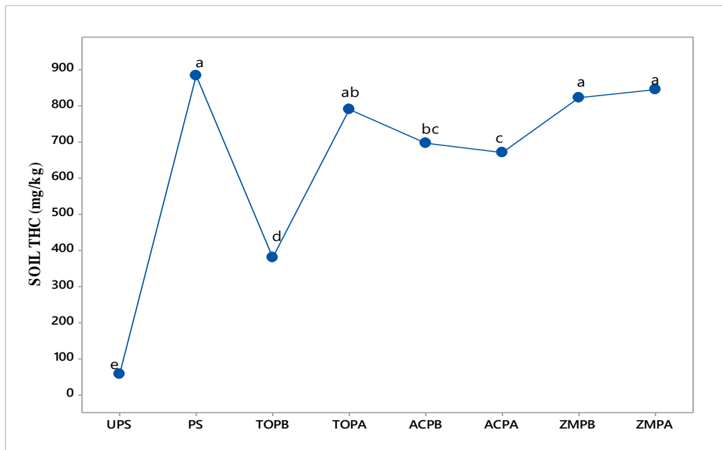
Fig. 4. Total Hydrocarbon Content for polluted and unpolluted soil samples at day 28 according to their pollution time
