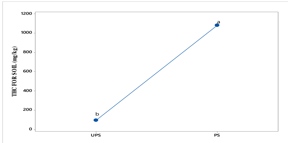
Fig. 2. Total Hydrocarbon Content for polluted and unpolluted soil samples at day zero The values reflect the mean and standard deviation of three replicates. Means differ considerably at ( p < 0.05 ) when they do not share a letter
