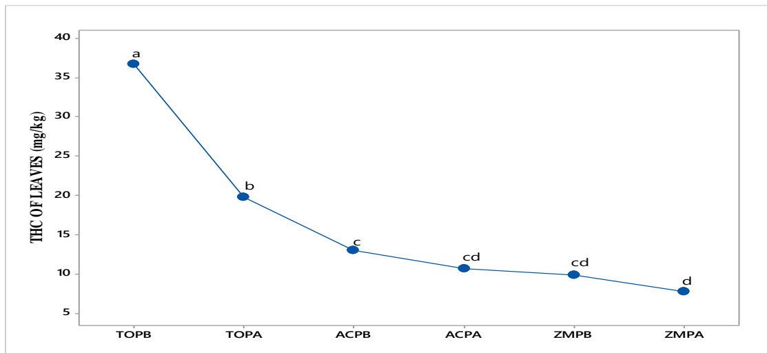
Fig. 6. Total Hydrocarbon Content for polluted test plants at day 28 according to their pollution time
