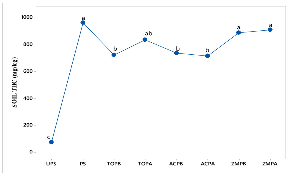
Fig. 3. Total Hydrocarbon Content for polluted and unpolluted soil samples at day 14 according to their pollution time
