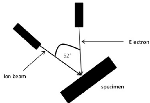
Fig. 1. A schematic diagram of the dual FIB/SEM. The angle between the FIB and SEM beams is 52°, with the ion beam at to the specimen
