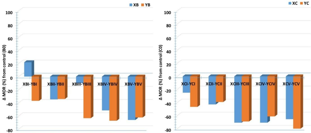
Fig. 4. MOR strength ( \Delta\% ) difference properties of experimental boards from controls
