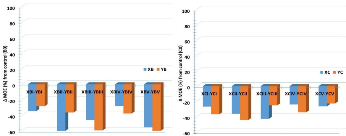
Fig. 5. MOE ( \Delta\% ) difference properties of experimental boards from controls
