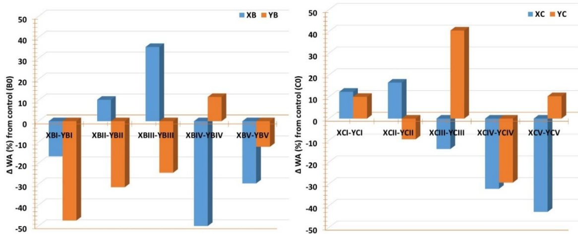
Fig. 1. Water absorption (Δ%) difference properties of experimental boards from controls
