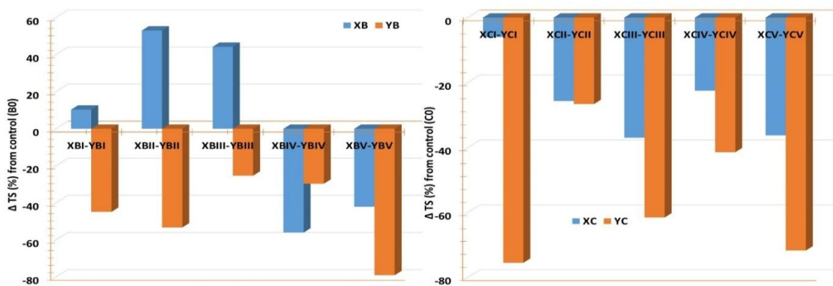
Fig. 2. Thickness swelling ( \Delta\% ) difference properties of experimental boards from controls
