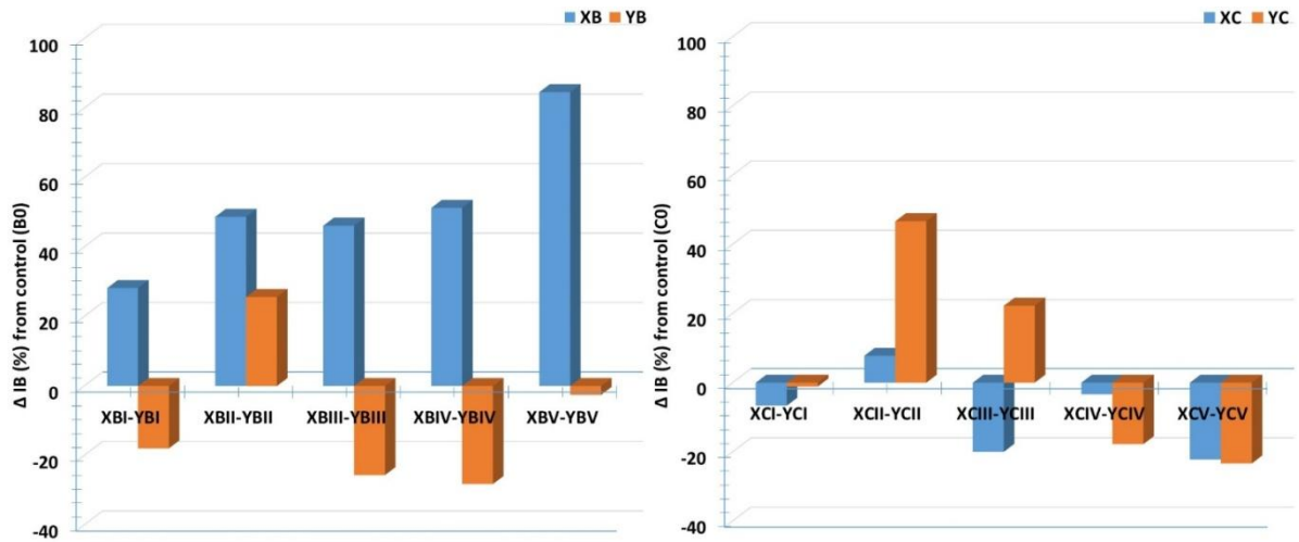
Fig. 3. IB strength ( \Delta\% ) difference properties of experimental boards from controls
