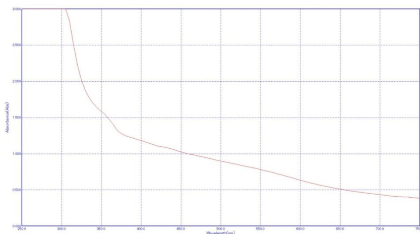
Fig. 2. UV spectroscopy
