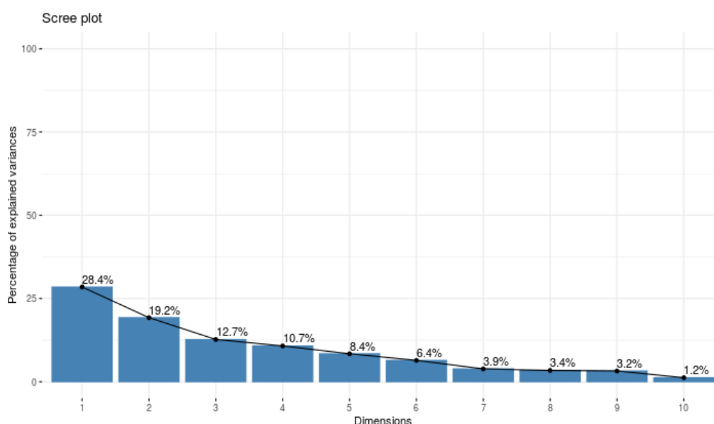
Fig. 1. Scree plot of Percentage Variance After PCA
