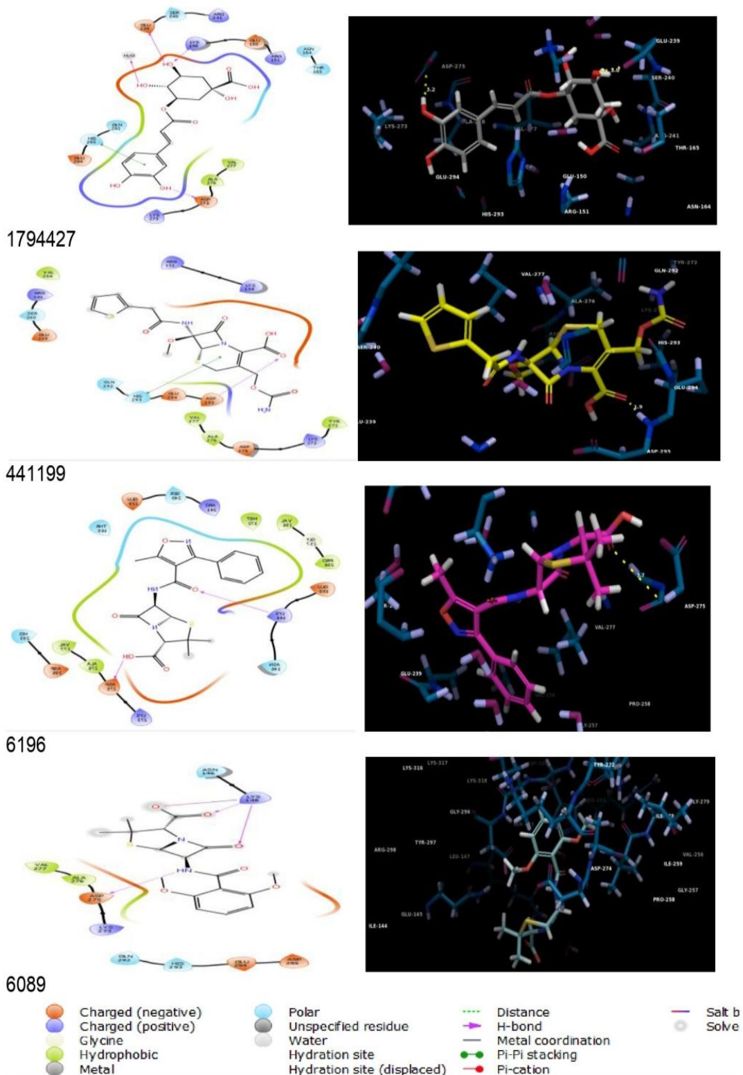
Fig. 1. 2 and 3D representation of the lowest binding energies of phyto ligand of Honey and standard drugs against Staphylococcus aureus (a). PBP2a(5M19); (b). Chlorogenic acid + PBP2a; (c). Cefoxitin,+ PBP2a; (d). Oxacillin + PBP2a
