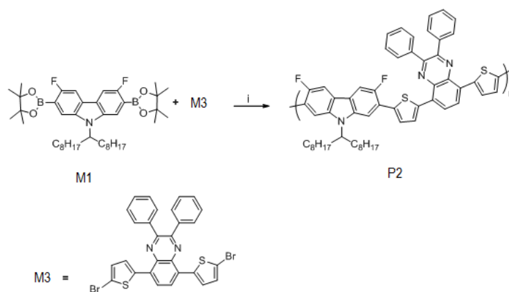
Scheme 2. Preparation of polymer P2 (i) Pd(AcO) 2 , tri- o -tolylphosphine, NaHCO 3 , THF
