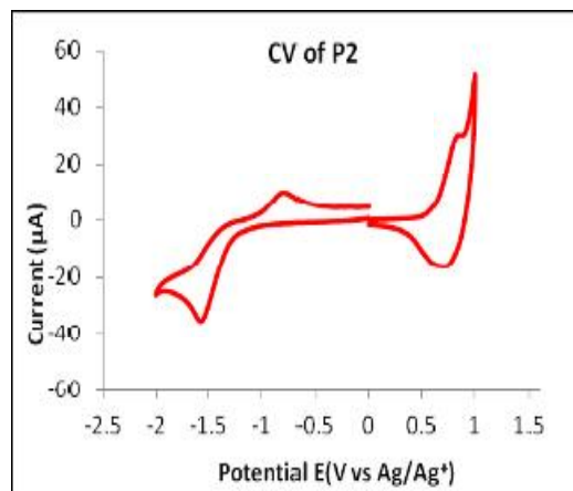
Fig. 4. Cyclic voltammograms of P2 films cast on platinum disc (0.00314 cm 2 ) in tetrabutylammonium perchlorate/acetonitrile at 100 mV/s
