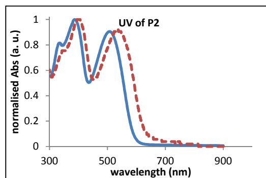
Fig. 2. Normalised absorption spectra of P2 in chloroform solution (blue line) and as thin film (brown line)
