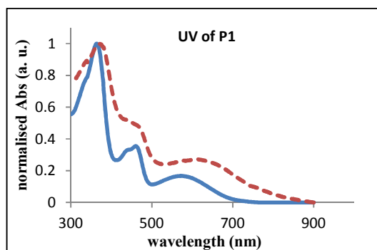
Fig. 1. Normalised absorption spectra of P1 in chloroform solution (blue line) and as thin film (brown line)
