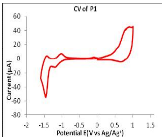
Fig. 3. Cyclic voltammograms of P1 films cast on platinum disc (0.00314 cm 2 ) in tetrabutylammonium perchlorate/acetonitrile at 100 mV/s
