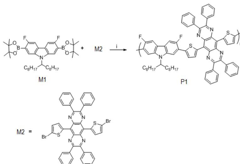
Scheme 1. Preparation of polymer P1 (i) Pd(AcO) 2 , tri- o -tolylphosphine, NaHCO 3 , THF
